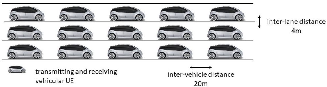
Figure 5: Highway Scenario
